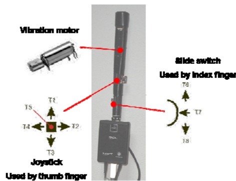
Figure 6. The Smart Cane user interface.
